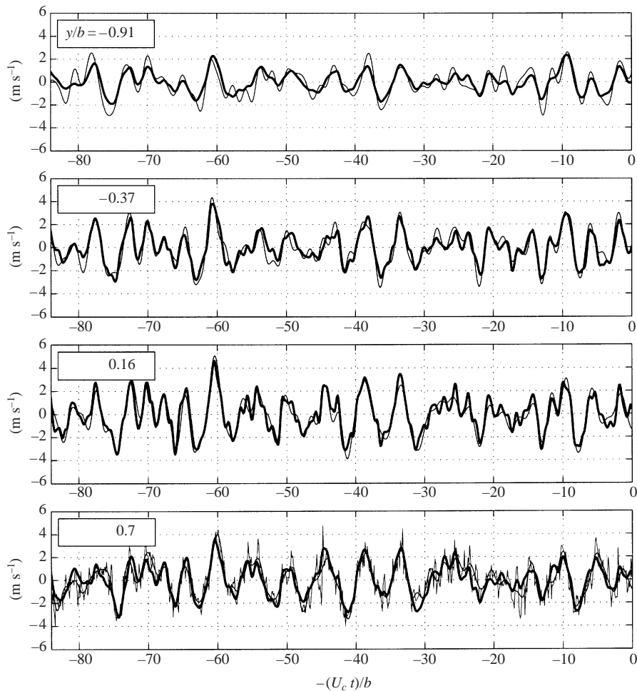
FIGURE 12. Filtered v -component velocity v_{direct}(y, t) (thin line) and the sum of the first two POD modes v_{POD}(y, t) (thick line) for several y -locations from the y -aligned rake experiment. The unfiltered instantaneous velocity v(y, t) is also shown in the y/b = 0.7 case for comparison.
