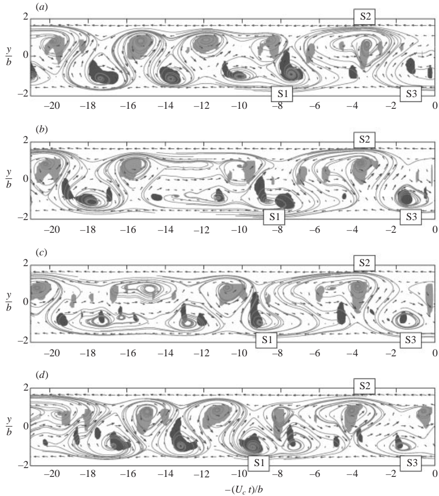
FIGURE 15. The velocity field (u, v) and pseudostreamlines of the reconstructed non-planar coherent structure u_z^{non-planar}(y, z, t) with the first N = 2 POD modes at (a) z/b = 1.4 , (b) 1.0, (c) 0.6 and (d) 0.2 spanwise locations from the z -aligned rake experiment. The regions of high spanwise vorticity |\omega_z| \geq 0.3U_m/b are shown as shaded regions, light grey – positive and dark grey – negative.
